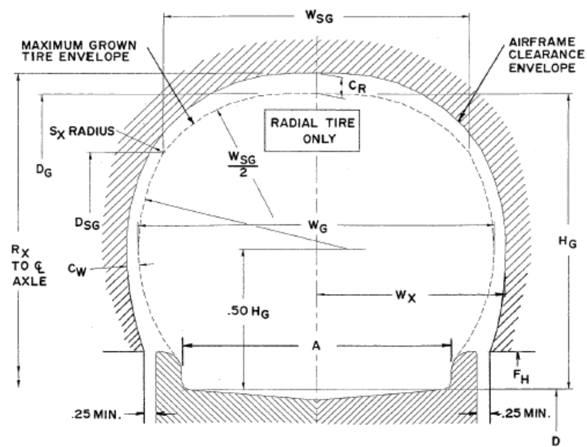
The above drawing represents clearances required for an unloaded free-spinning grown tire or a loaded grown tire above the axle centerline.
