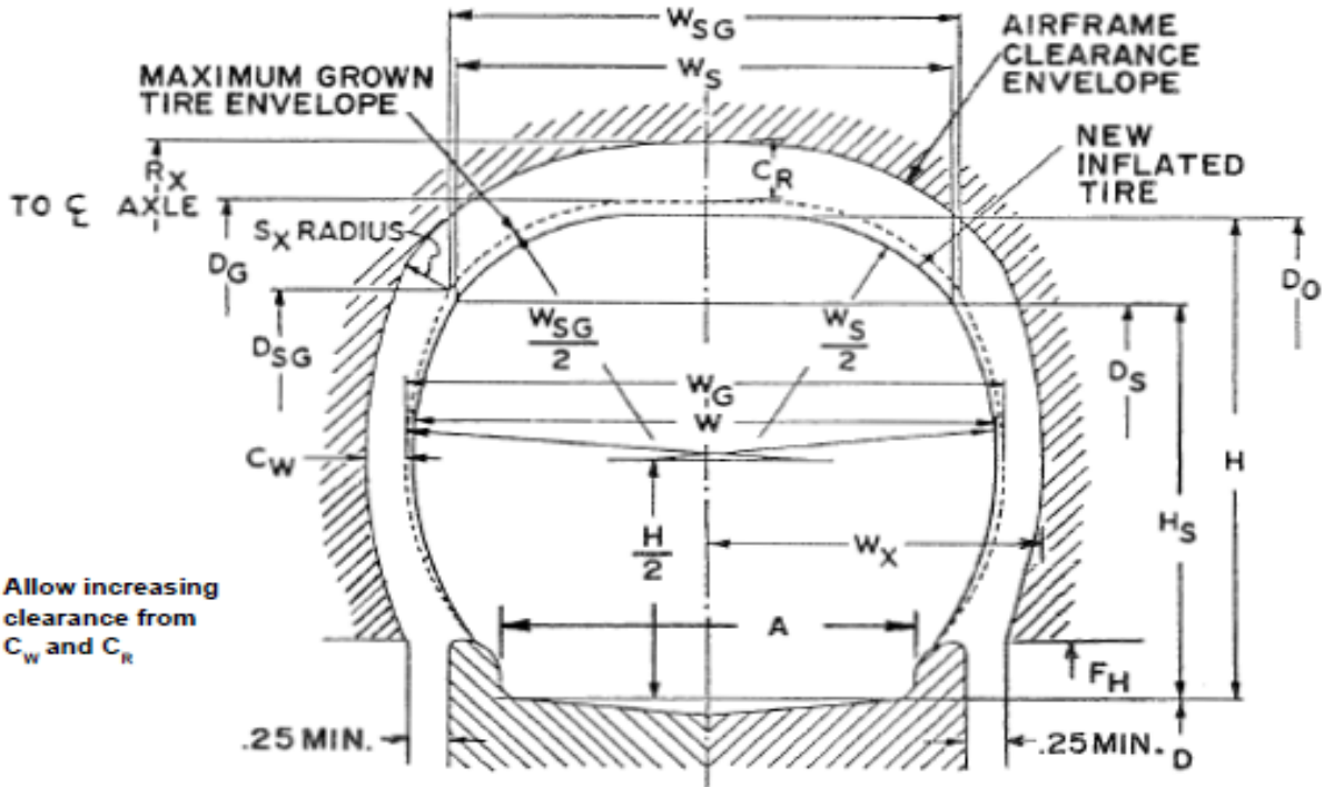
The above drawing represents clearances required for an unloaded free-spinning grown tire or a loaded grown tire above the axle centerline.
